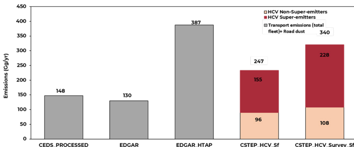
Figure 2: Comparison of India's transport emissions ( PM_{2.5} ) with the estimations of global EIs. The study estimate considers trucks' VKT as 300 km/day, which is the upper end for our emission estimate (The baseline VKT is 142 km/day.)
